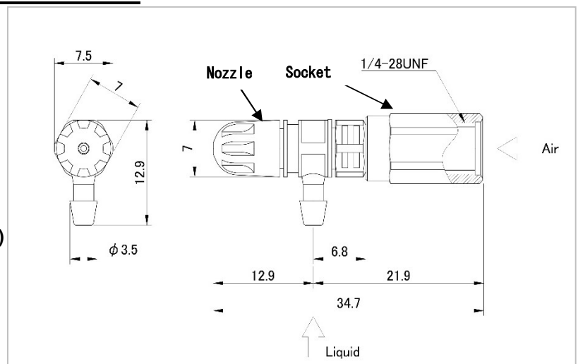
Siphon (self-feeding) spray with compressed air
